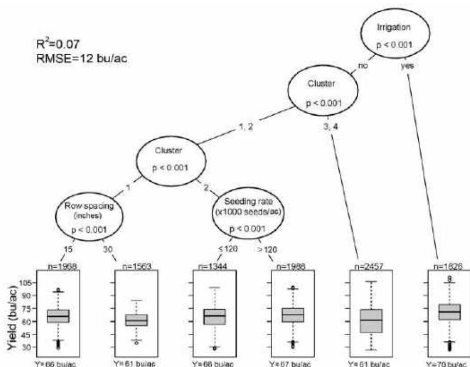
Figure 4. Conditional inference tree for soybean yields (bu/ac) as affected by environment (clusters) and management practices. In each boxplot, the central rectangle spans the first to the third yield quartiles. The solid line inside the rectangle is the mean which is also numerically shown at the bottom (Y). The number of data points comprising each mean is shown on top of each boxplot (n). The white circles show outlier yields.
